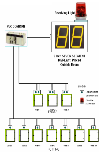
Oven Timer Monitoring System
